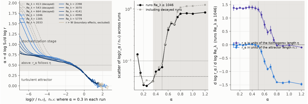
FIG. 11. Turbulent attractor and stochastization stage in the Max Planck data. Left: the measured index of each run against \log(r/r_{0.3}) , where r_{0.3} is the separation at which that run's index equals 0.3; dashed grey curves are the decayed-turbulence runs, Re_\lambda < 10^3 . Middle: the scatter of \log(r_\alpha/r_{0.3}) across the runs at fixed \alpha . Right: the Reynolds-number dependence of r_\alpha in units of the Kolmogorov length and of r_{0.3} (runs Re_\lambda \geq 1046 ). In the turbulent attractor, \alpha < 0.355 (white), the runs collapse tightly (scatter below 0.05, dashed line); in the stochastization stage (grey) the scatter grows, slowly up to \alpha \approx 0.5 (dotted lines) and steeply above, where r_\alpha follows \eta . The tan ends of the curves are the boundary-effects region r > W , not used.
