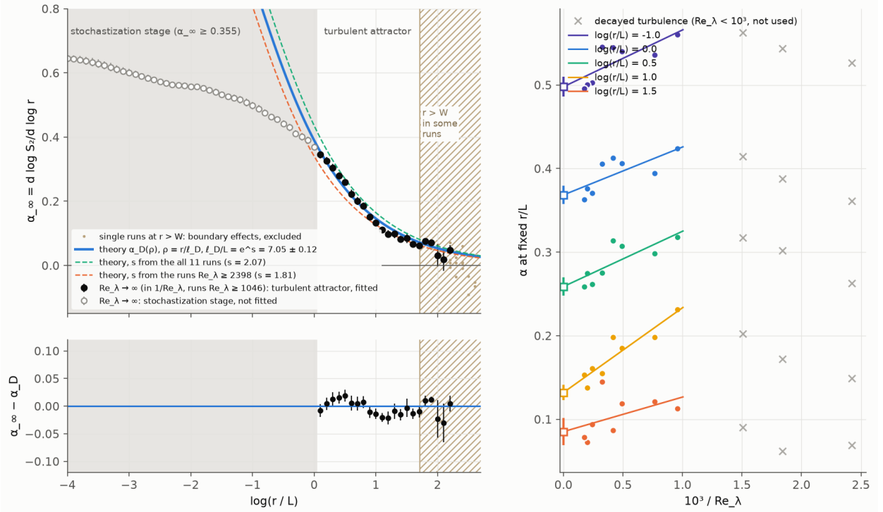
FIG. 9. Left: the Max Planck index extrapolated to Re_\lambda \rightarrow \infty in 1/Re_\lambda (runs Re_\lambda \geq 1046 ) against the odd-ensemble theory with one scale parameter (blue). Filled circles: the turbulent attractor, \alpha_\infty < 0.355 , to which the theory is fitted; open grey circles: the stochastization stage (grey band), not fitted. Dashed lines use the shifts fitted to the extrapolations with all runs and with Re_\lambda \geq 2398 only. The residuals are shown below. Right: \alpha_{\text{exp}} against 1/Re_\lambda at fixed r/L ; squares are the extrapolated values, grey crosses the decayed-turbulence runs, which are not used. The hatched band starts where the first run reaches r = W ; small tan dots are the single-run values at r > W (boundary effects), which are not used either.
