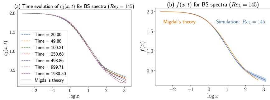
FIG. 10. Effective index \langle r \partial_r \log(\Delta v^2) \rangle of the 4096^3 DNS of decaying turbulence by Rodhiya and Sreenivasan [11] (Birkhoff-Saffman initial spectrum) against the Euler-ensemble prediction (from Ref. [5]).
