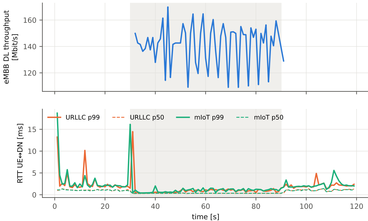
eMBB load phase (shaded): 2 UEs \times 4 TCP streams, slice MBR 150 Mbit/s
