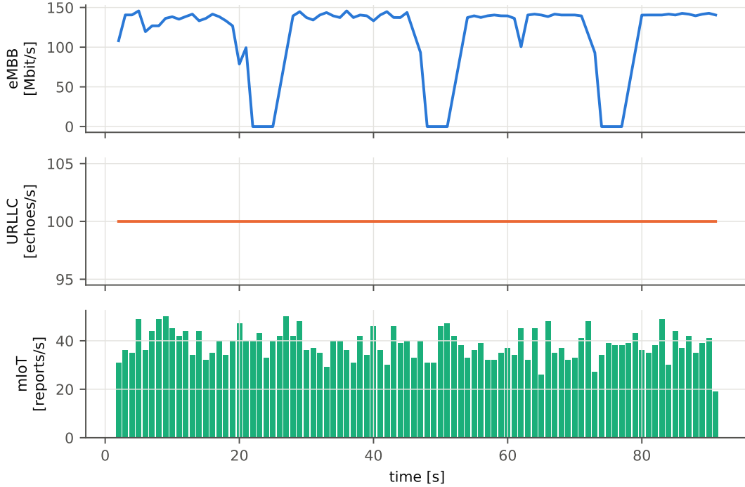
Figure 5: Per-slice offered traffic in scenario S1 (E6).
