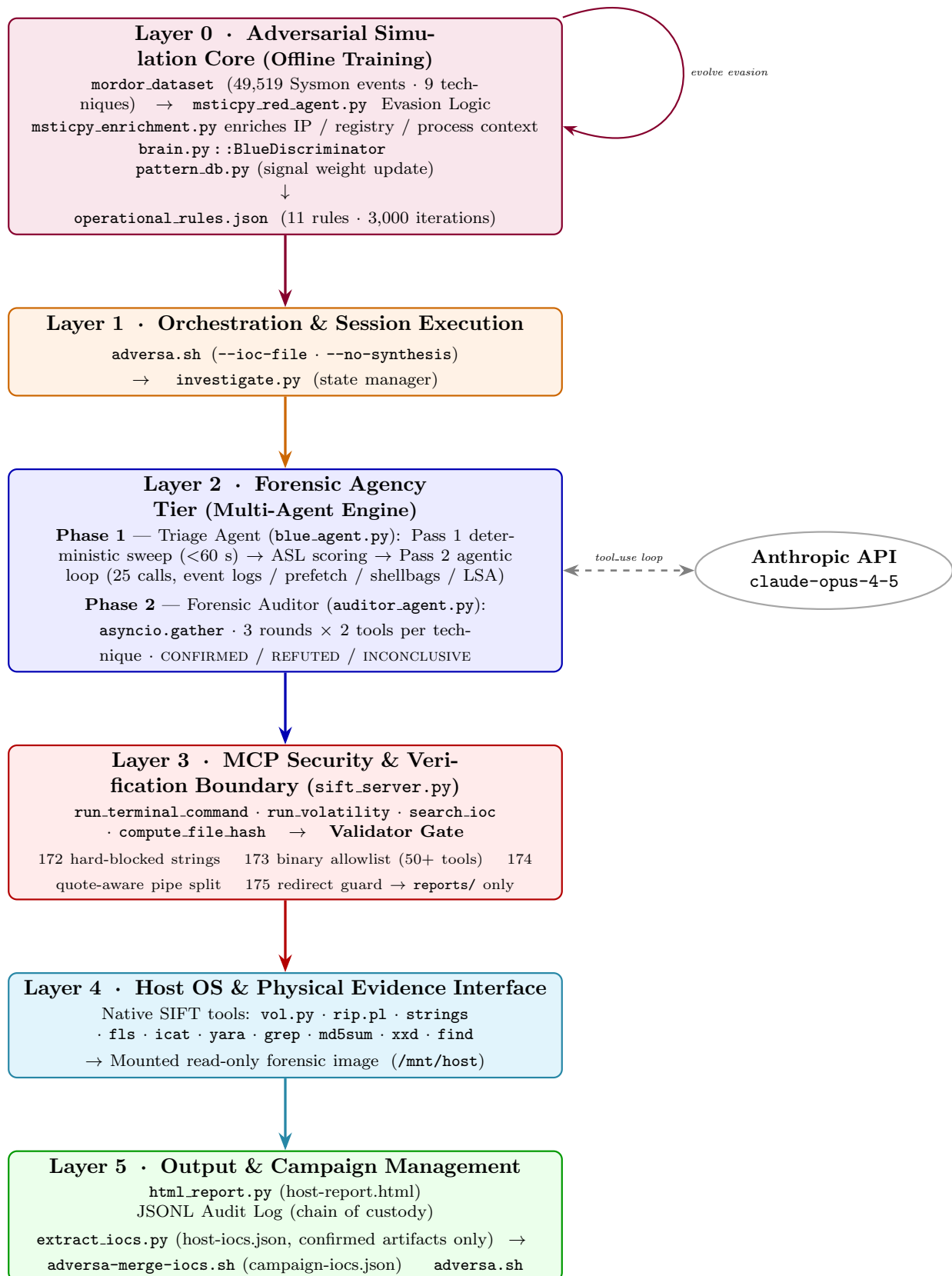
Figure 1: AdversA Layered Forensic Architecture Stack
