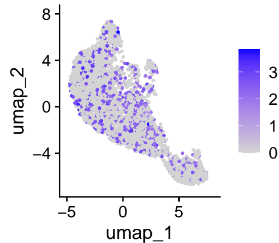
RRAD
