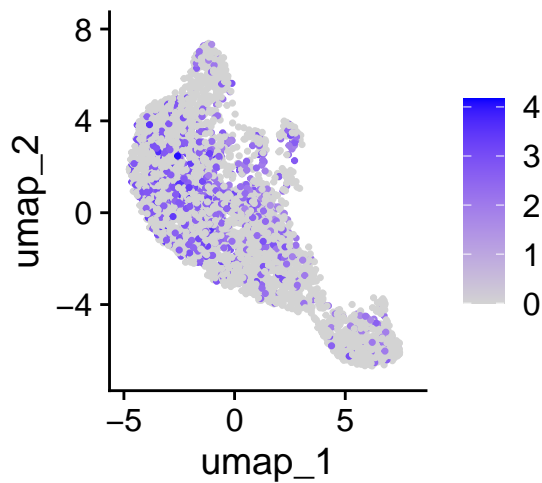
KRT6B
