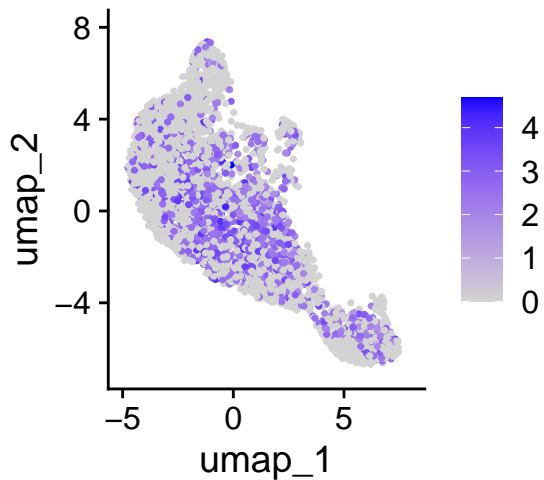
CRABP2
