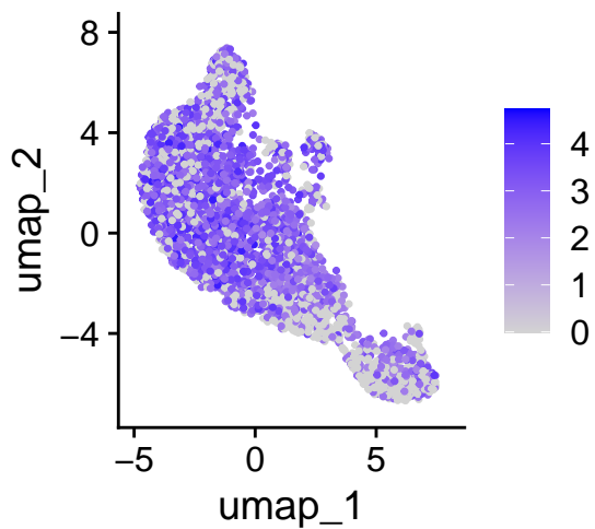
CRABP2
