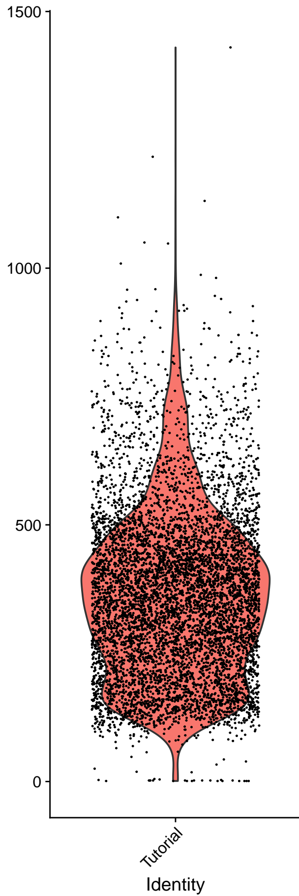
nFeature_RNA
