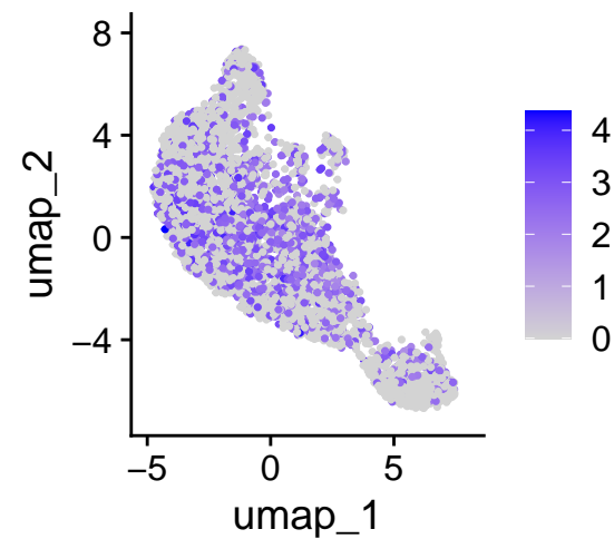
RRAD
