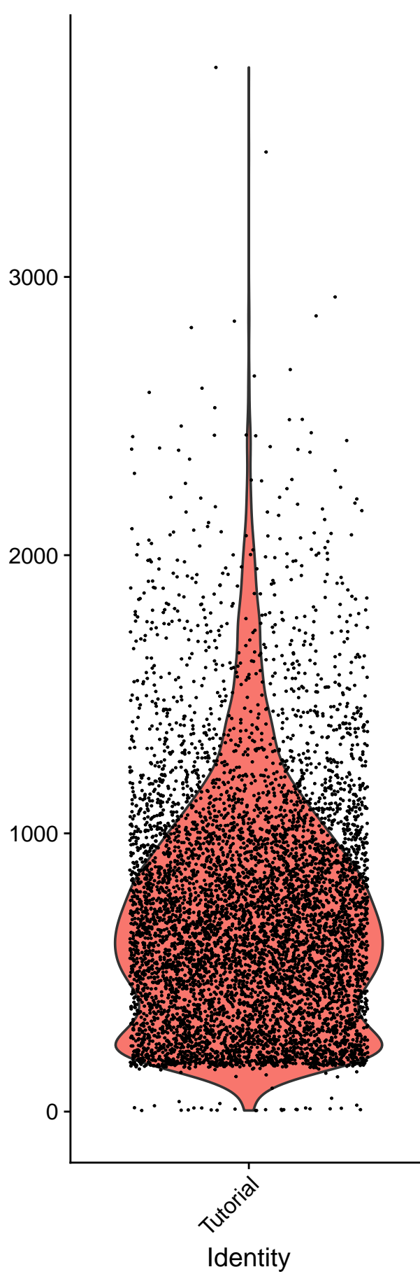
nCount_RNA
