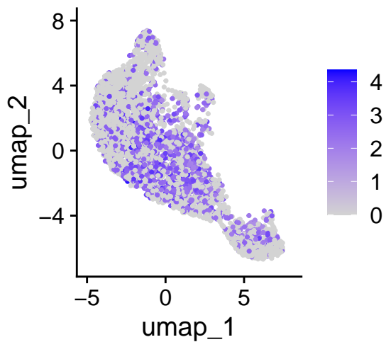
KRT6C
