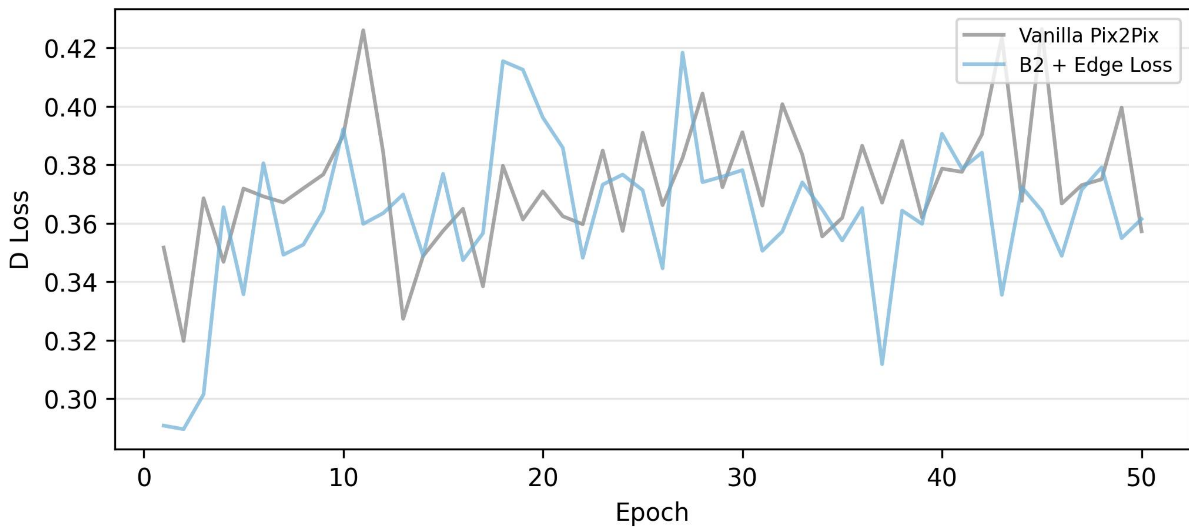
(b) Discriminator Loss
