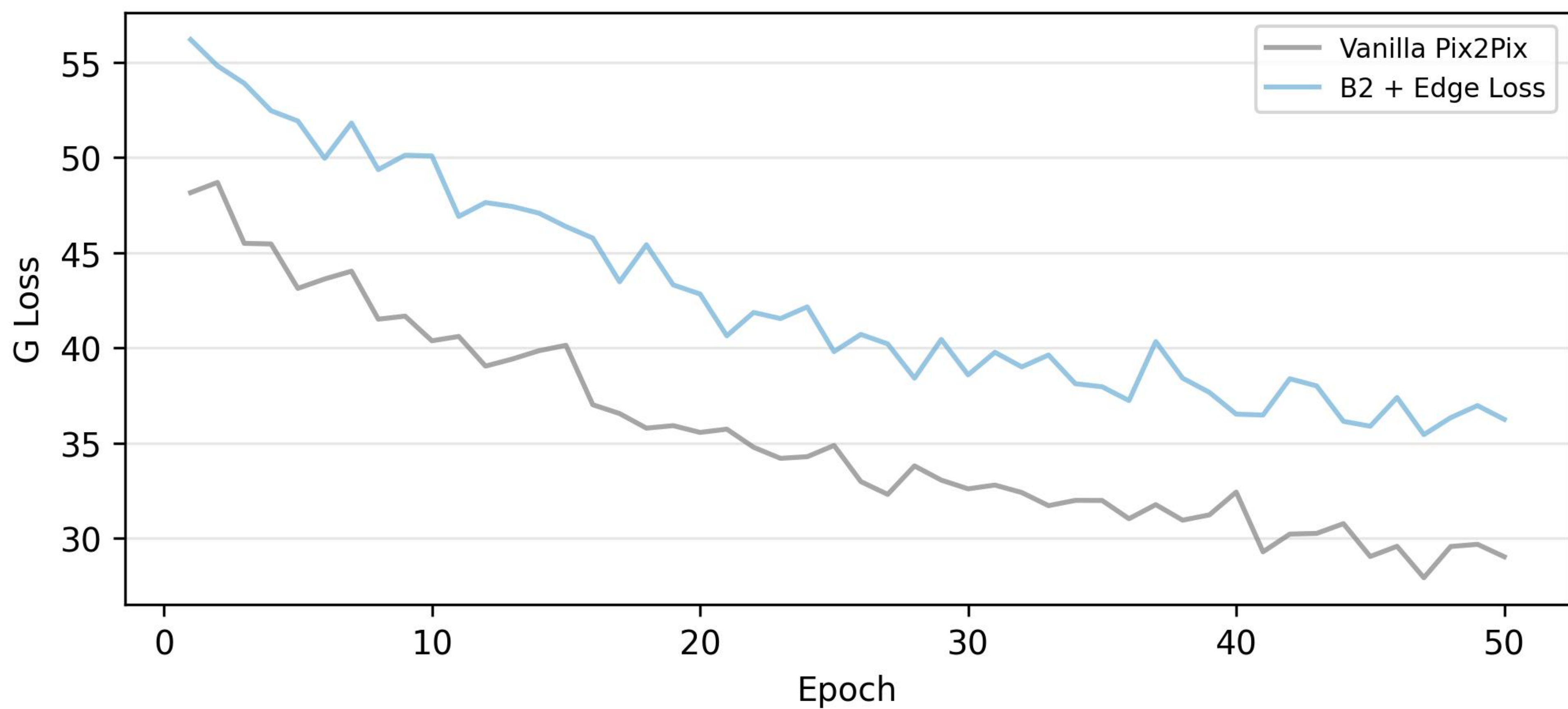
(a) Generator Loss
