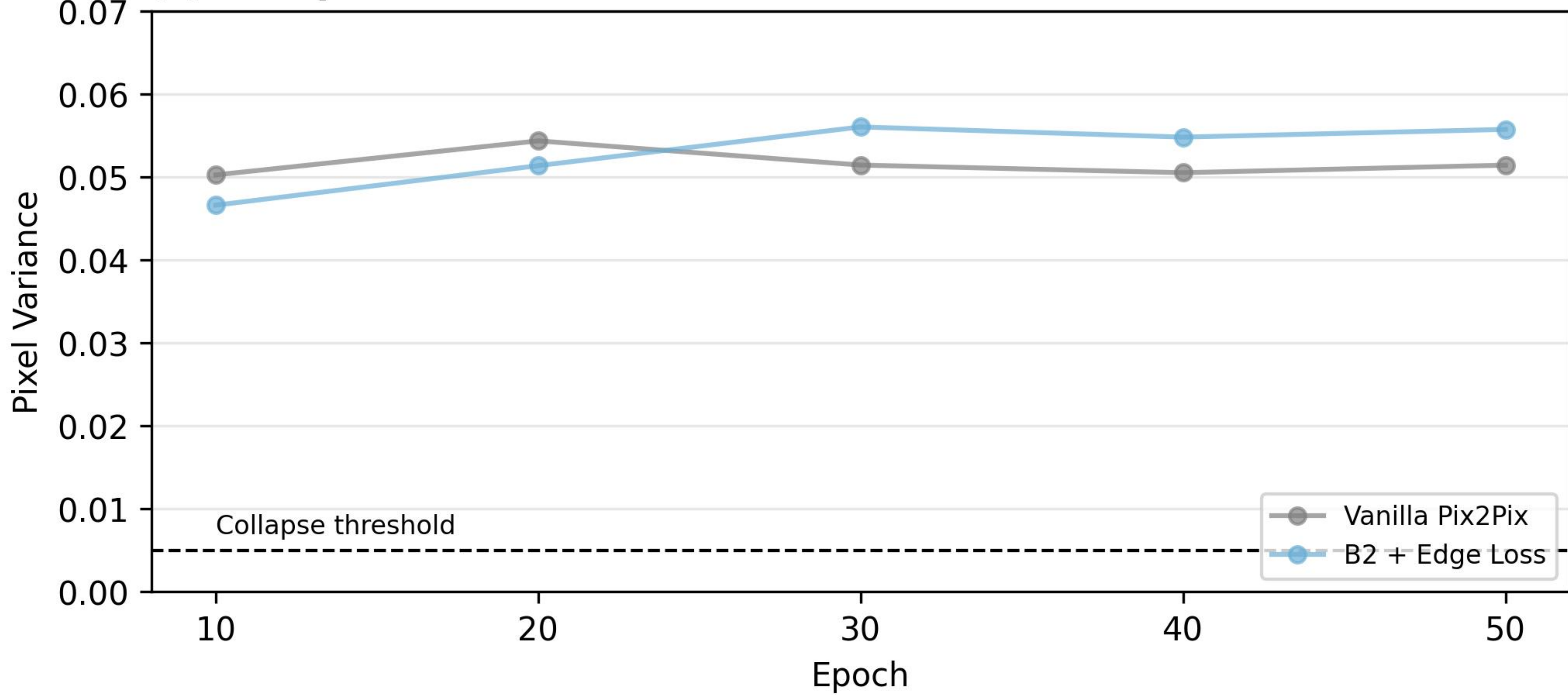
(c) Collapse-Check Variance
