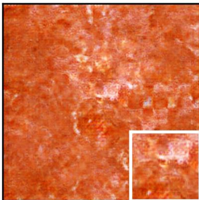
Vanilla Pix2Pix
