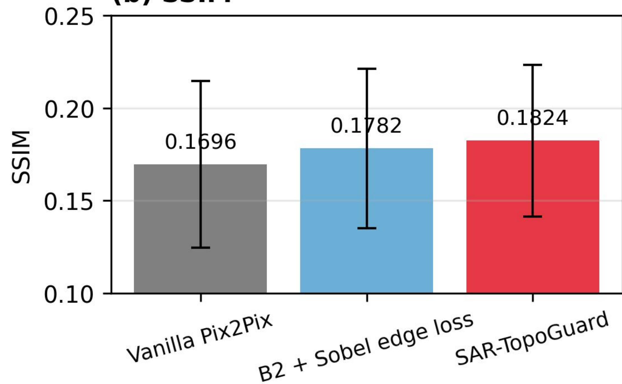
(b) SSIM
