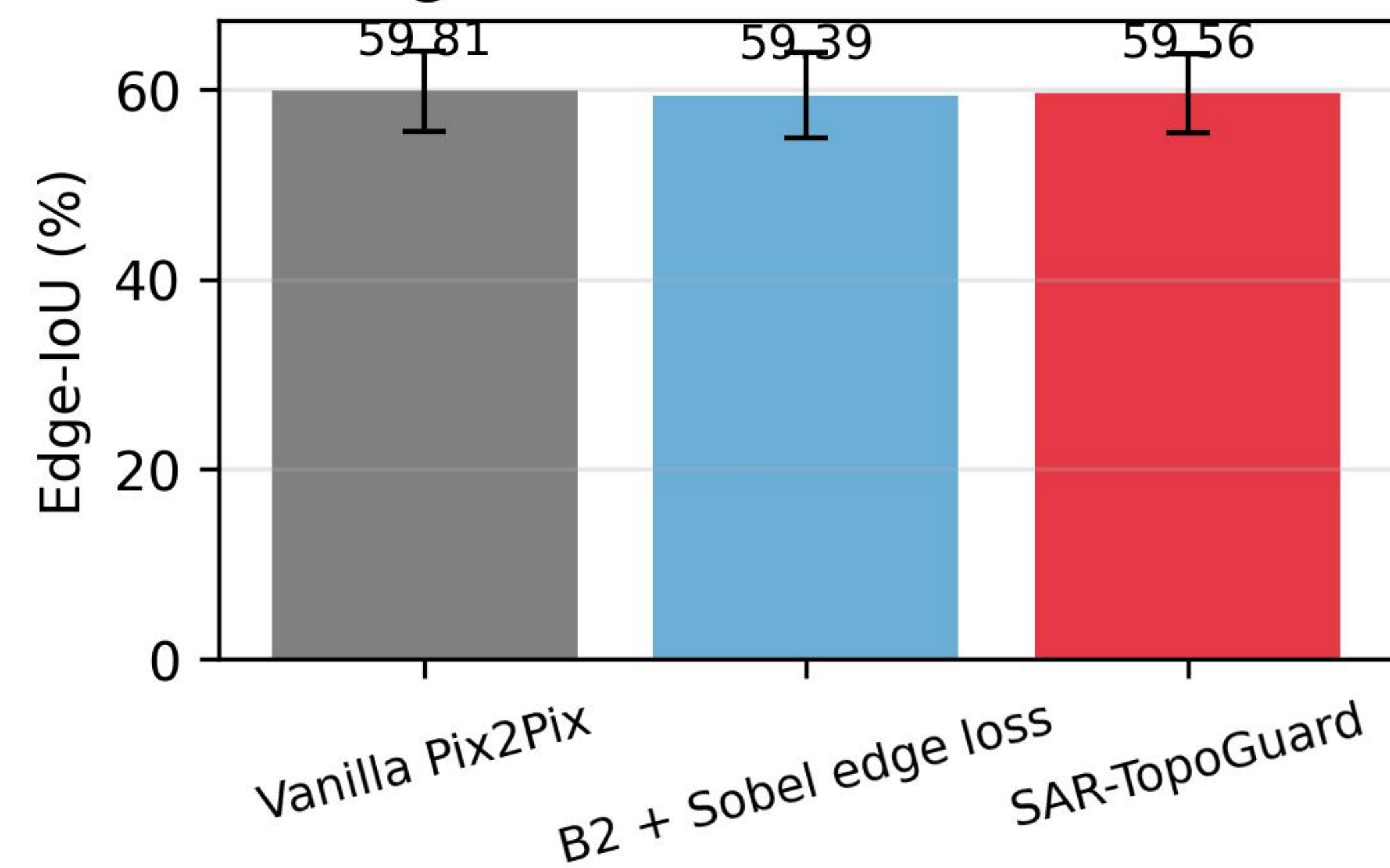
(c) Edge-IoU
