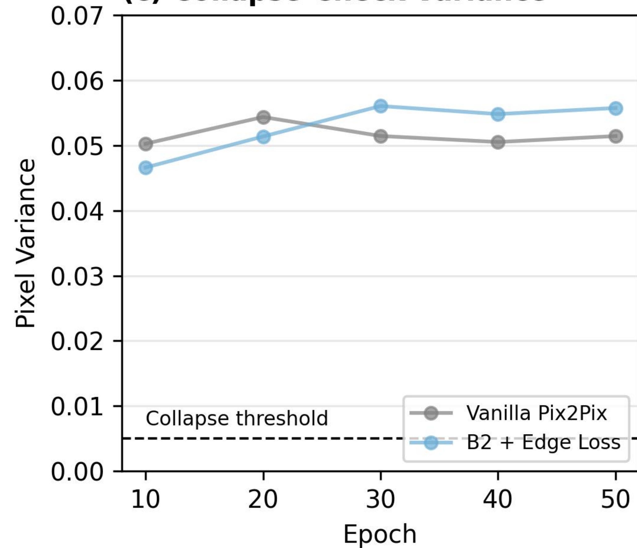
(c) Collapse-Check Variance
