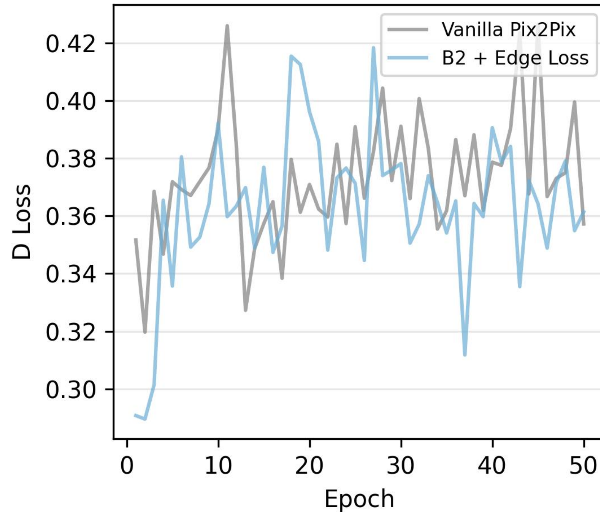
(b) Discriminator Loss
