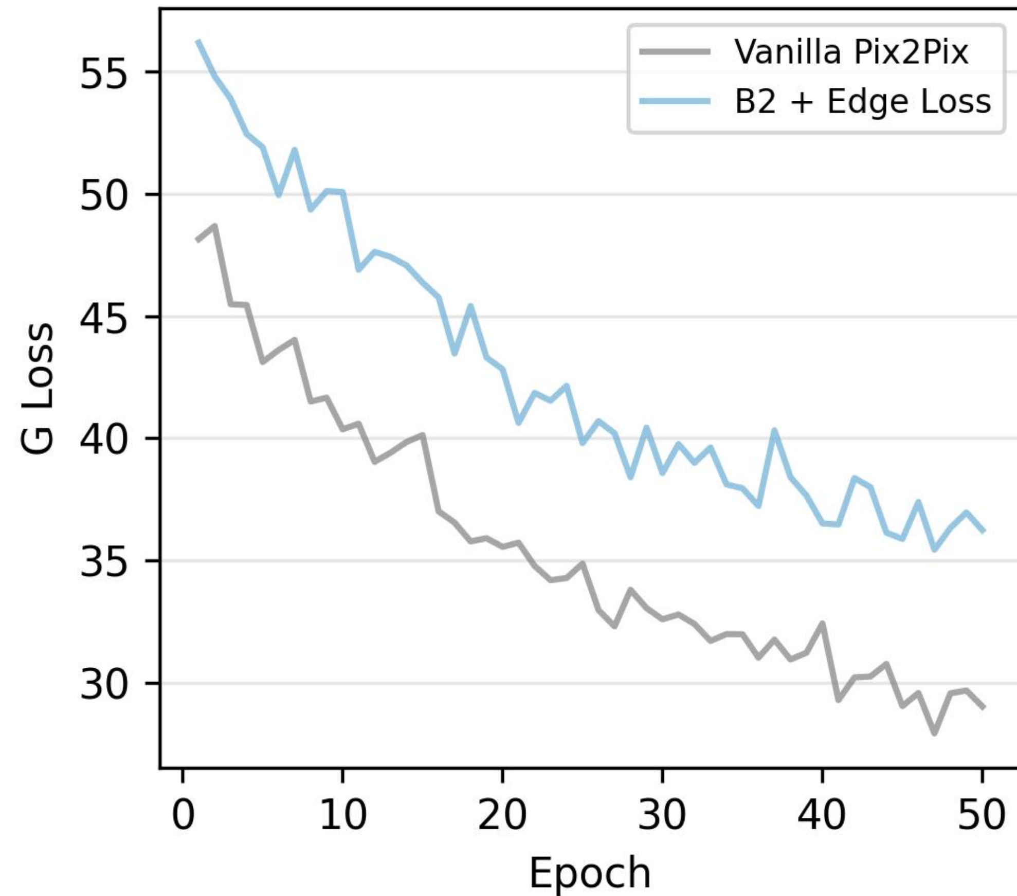
(a) Generator Loss
