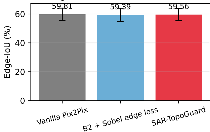
(c) Edge-IoU
