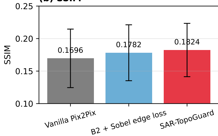
(b) SSIM
