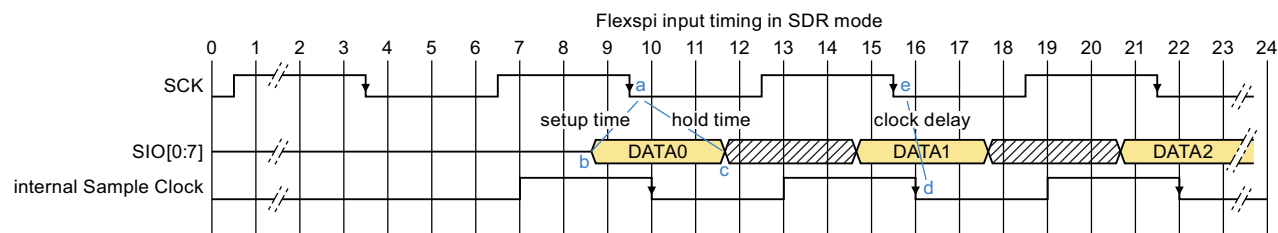
Figure 19. FlexSPI input timing in SDR mode where FlexSPI in _MCR0[RXCLKSRC] = 0X0, 0X1
