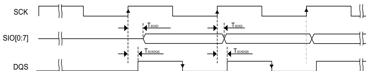
Figure 20. FlexSPI input timing in SDR mode where FlexSPI in _MCR0[RXCLKSRC] = 0X3 (case A1)
