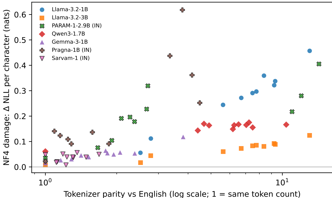
Tokenizer tax vs 4-bit quantization damage 7 models × 11 languages, Spearman \rho = 0.71
