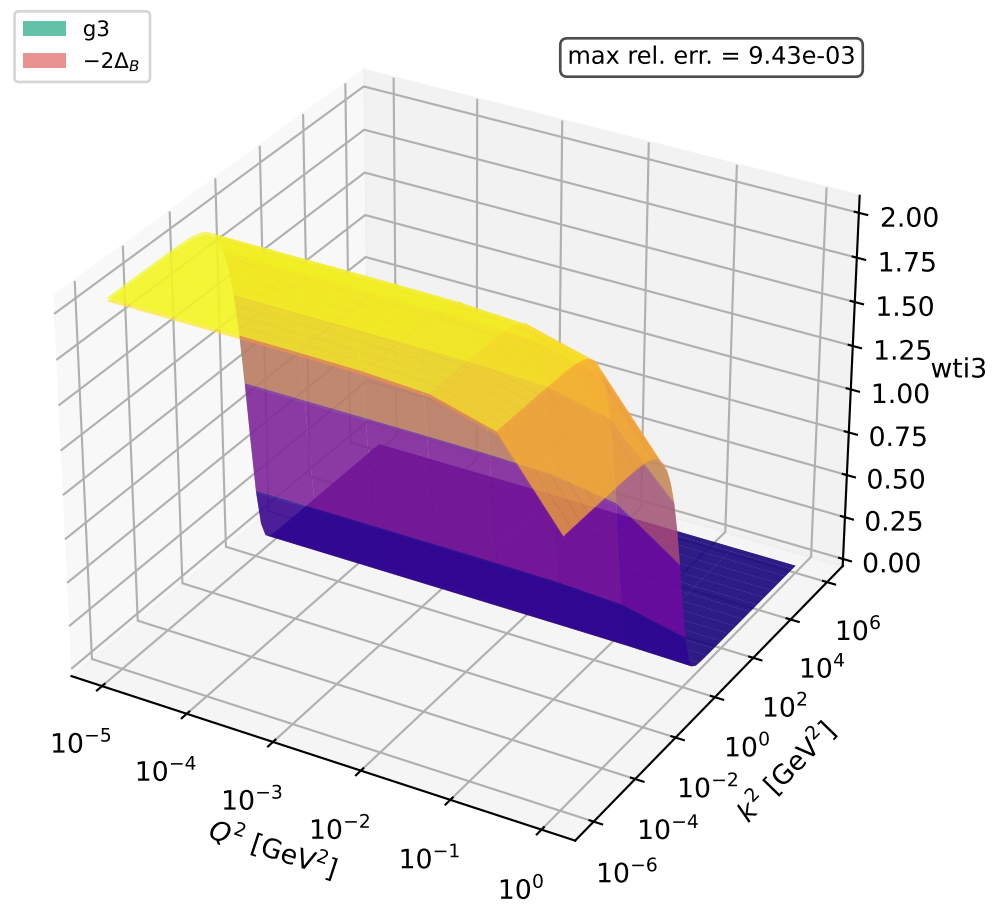
WTI 3: g_3 vs -2\Delta_B
