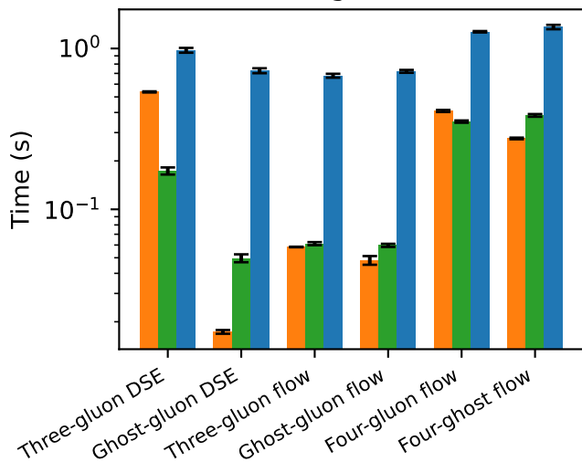
Yang-Mills
