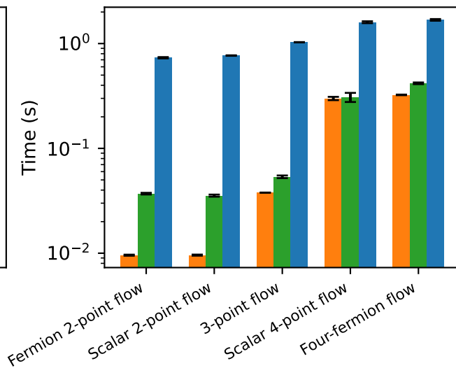
Yukawa
