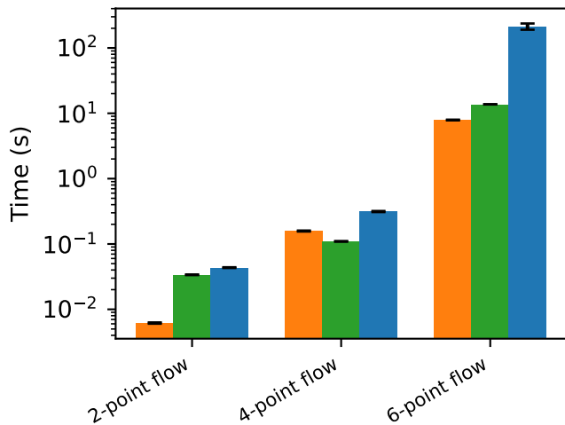
Yang-Mills
