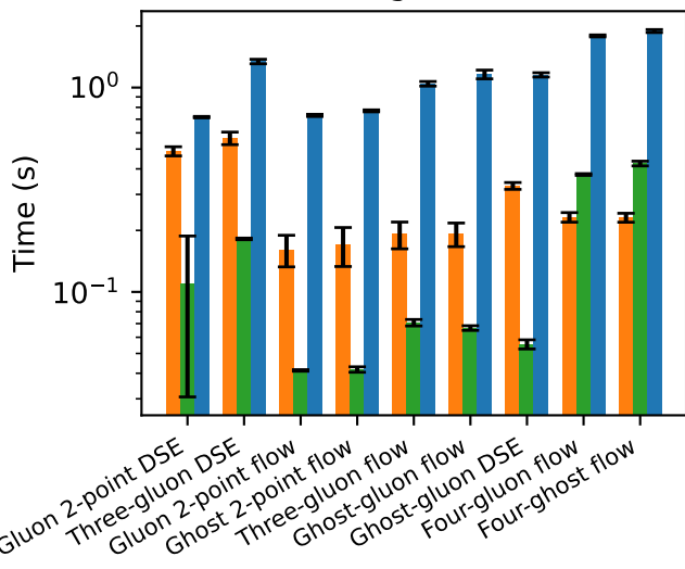
Yang-Mills
