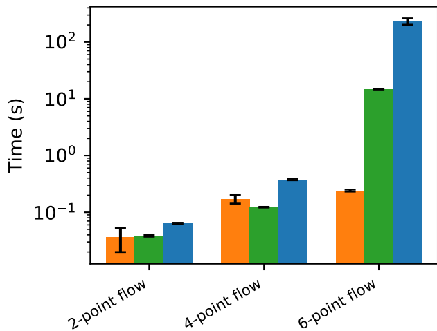
Yang-Mills
