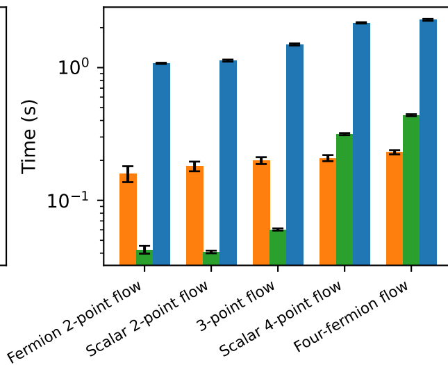
Yukawa
