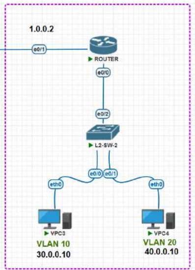
ROUTER ON-A-STICK
