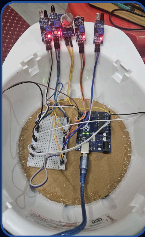
Internal Embedded Assembly
