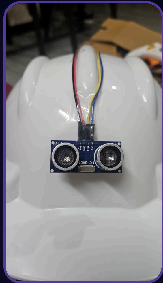
External Sensor Layout
