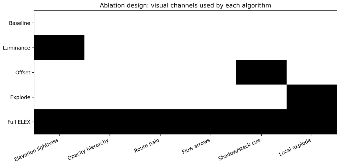
Figure 3. Ablation matrix showing which visual channels each algorithm variant uses.
