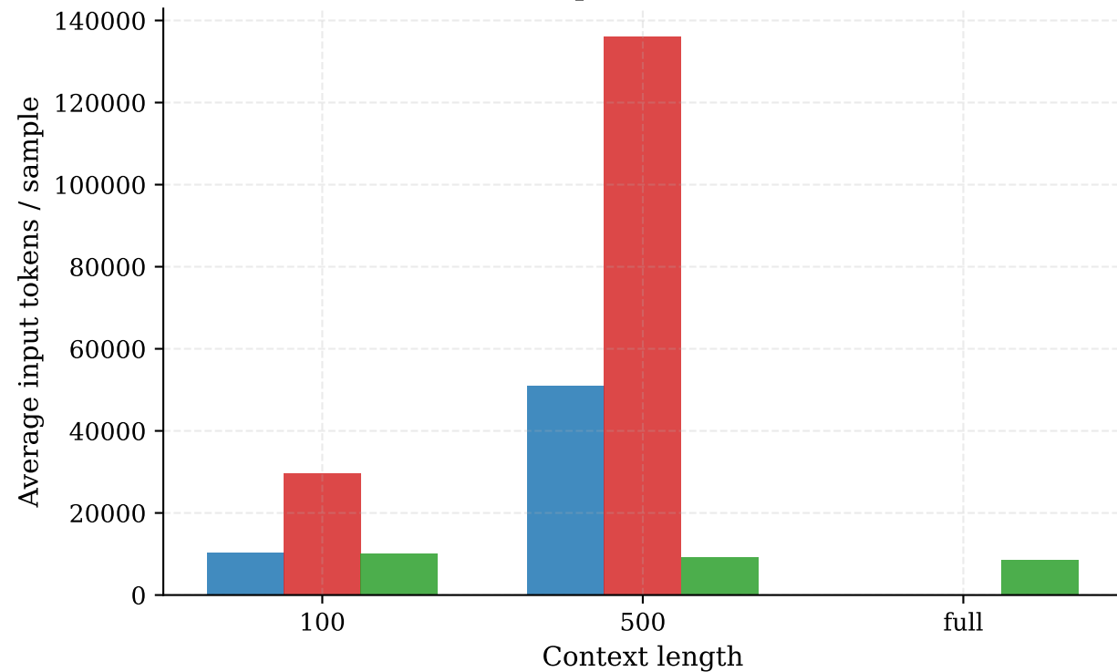
Average input/output tokens vs context (openai/gpt-5-mini)
