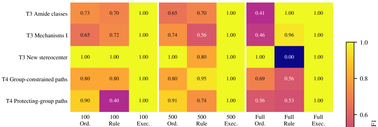
Qwen 3.5
