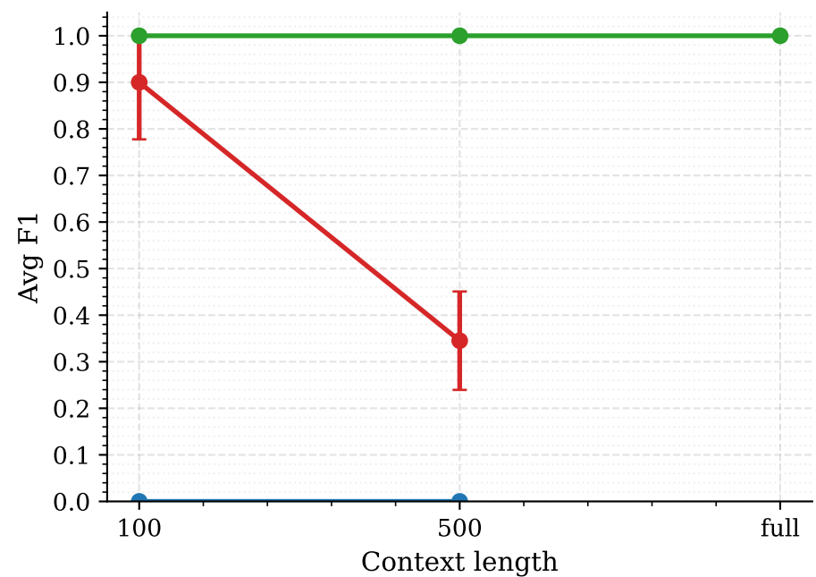
Combined MW and Ring Change
