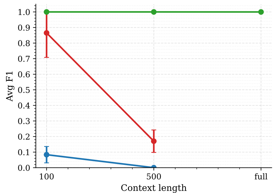
Ring Count Change
