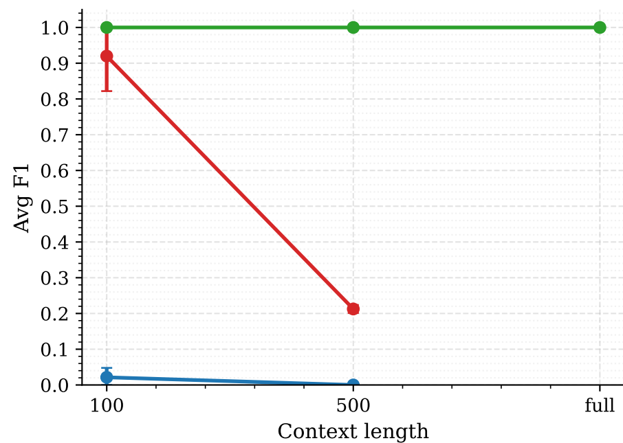
Aromatic Ring Formation
