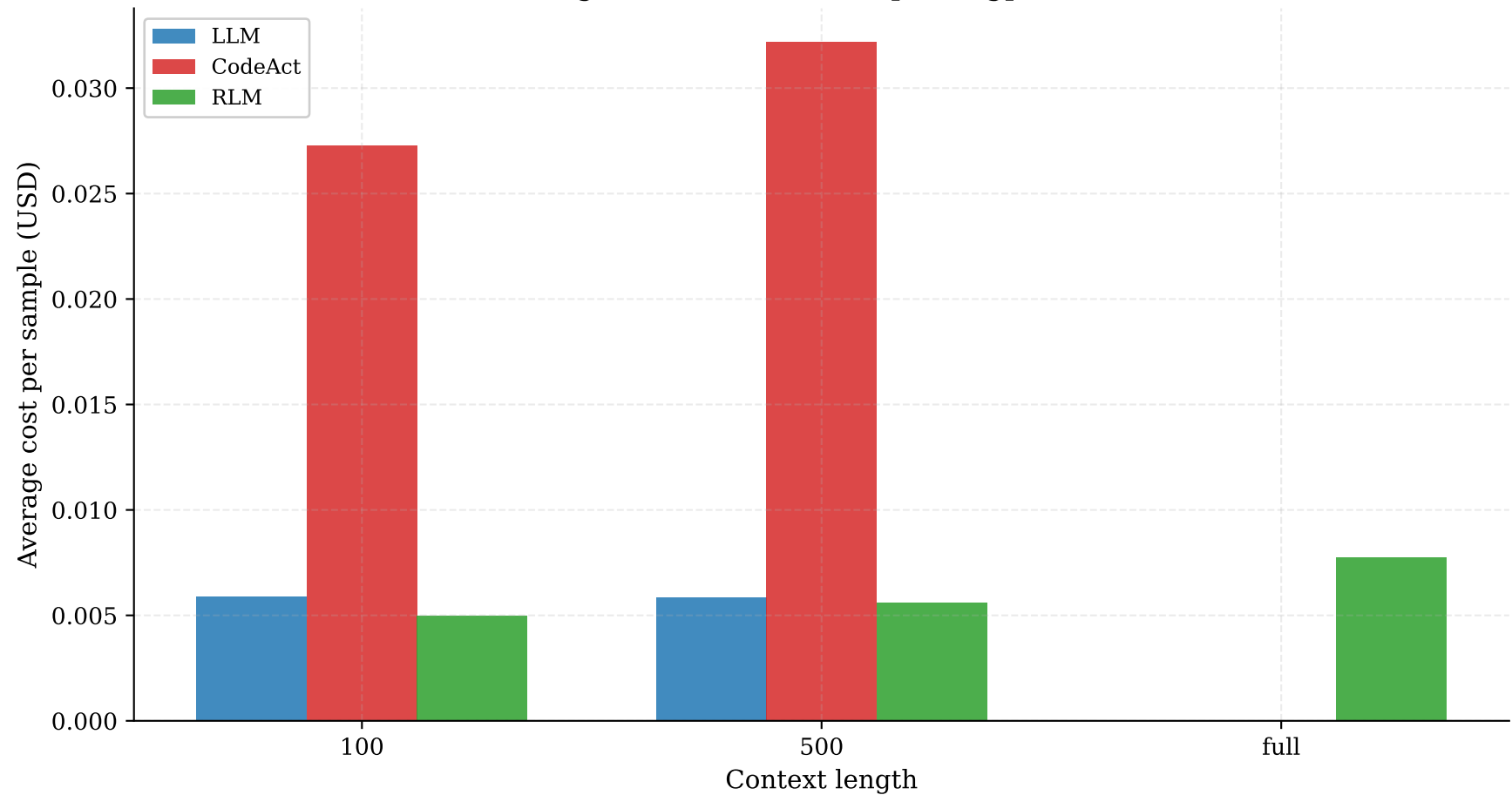
Average cost vs context (openai/gpt-5-mini)
