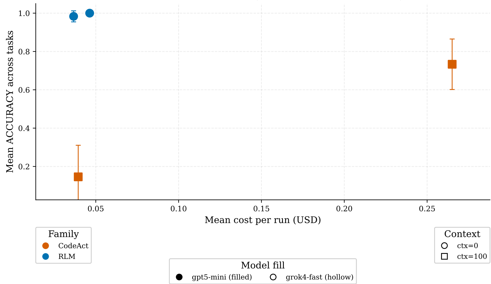
Mean ACCURACY vs cost (error bars = across-task std)
