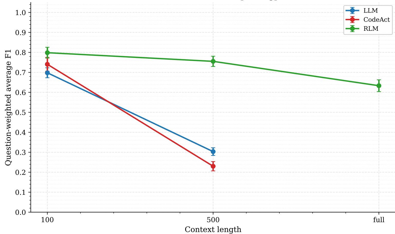
Tier3 overall F1 vs context (openai/gpt-5-mini)
