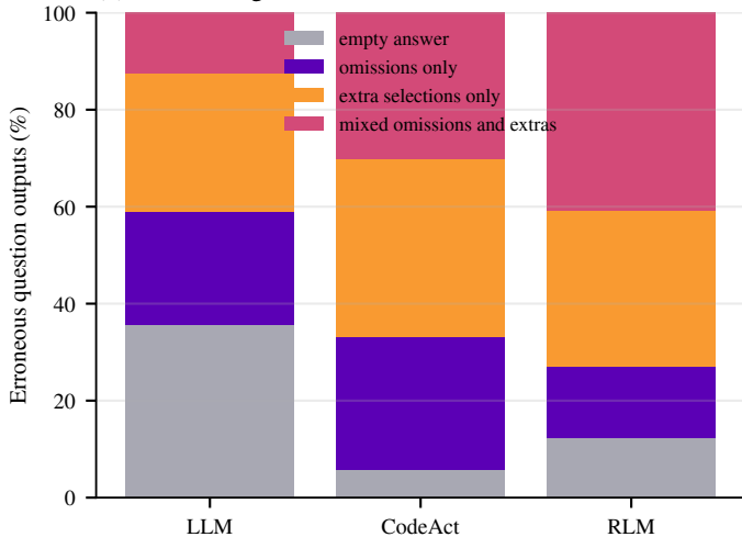
(b) Set-error signatures in retained traces
