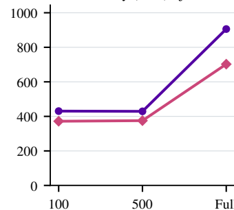
Peak memory (MiB) / job
