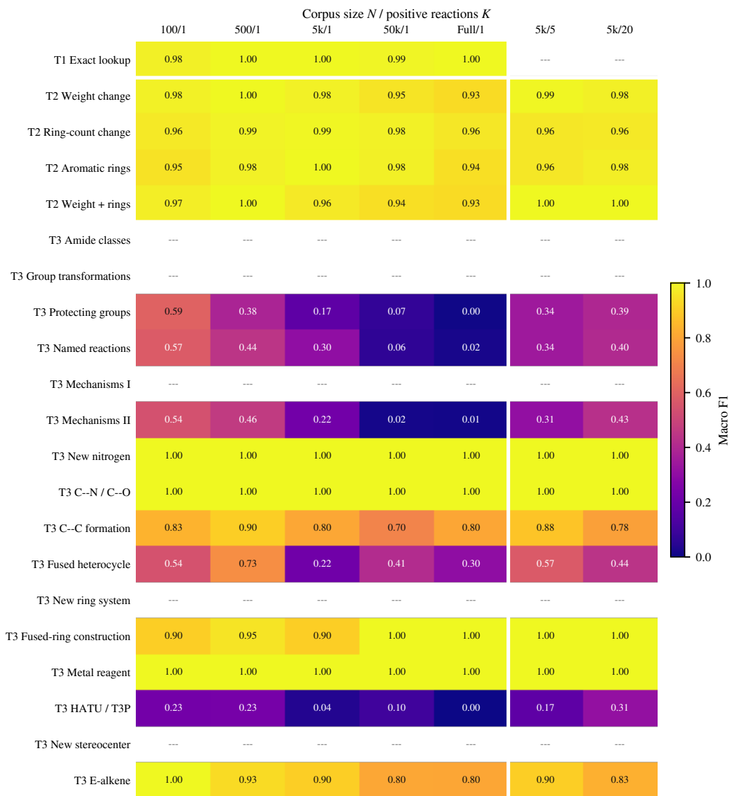
Figure 4: GPT-5 mini matched-cardinality macro-F1 by task. The first five columns increase corpus size N with one positive reaction ( K = 1 ); the final two hold N = 5,000 and increase K . Each cell averages five repetitions. Tier 1 was evaluated only in the fixed- K scale sweep.
