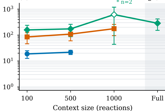
(c) Tier 3: Reaction-level reasoning ( n=35 )
