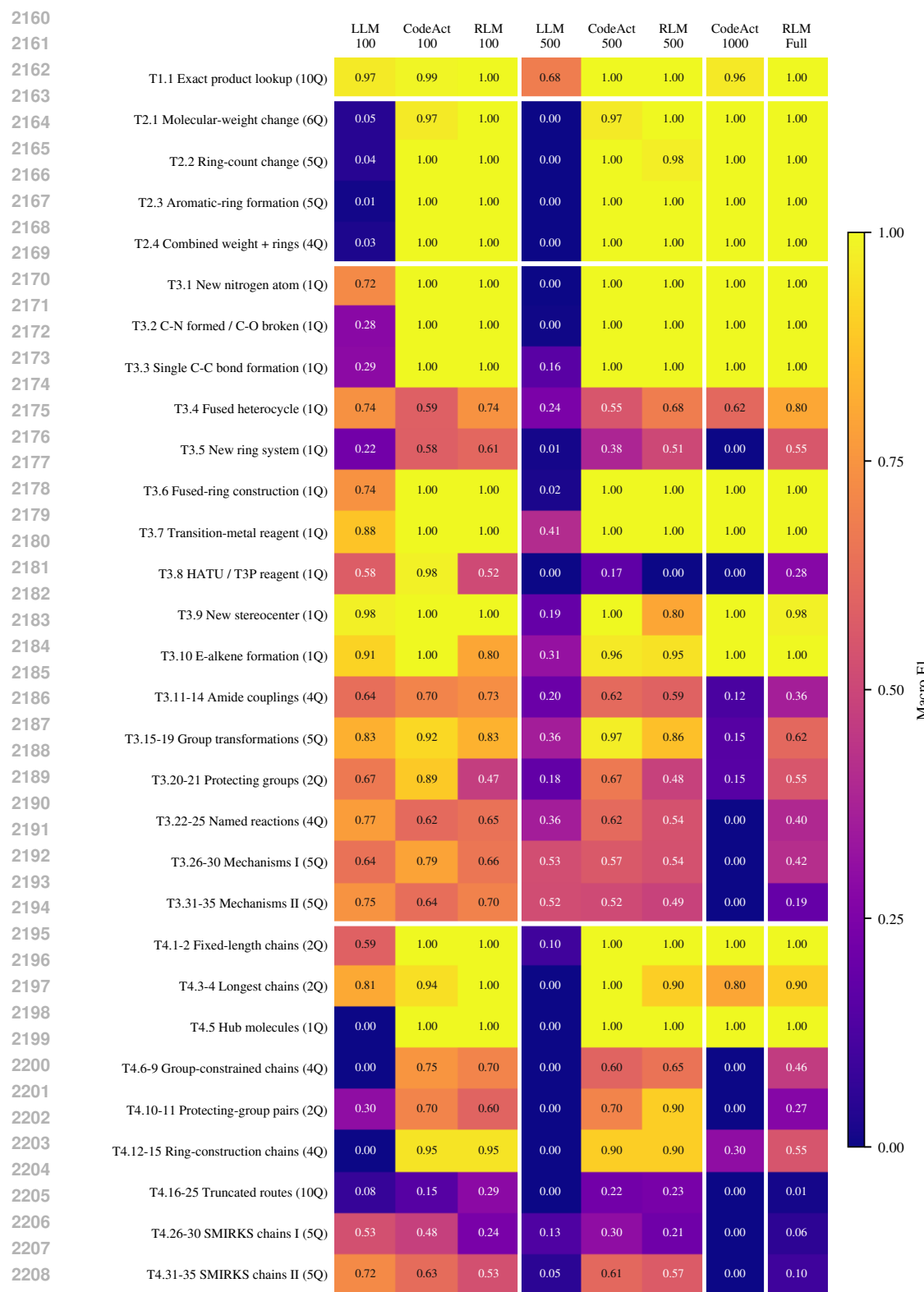
Figure 31: GPT-5 mini task-level macro-F1, averaged across five repetitions. Terminal failures contribute zero. The heatmap preserves all 30 task configurations and includes the x = 1000 CodeAct extension; full-corpus access is RLM-only.
