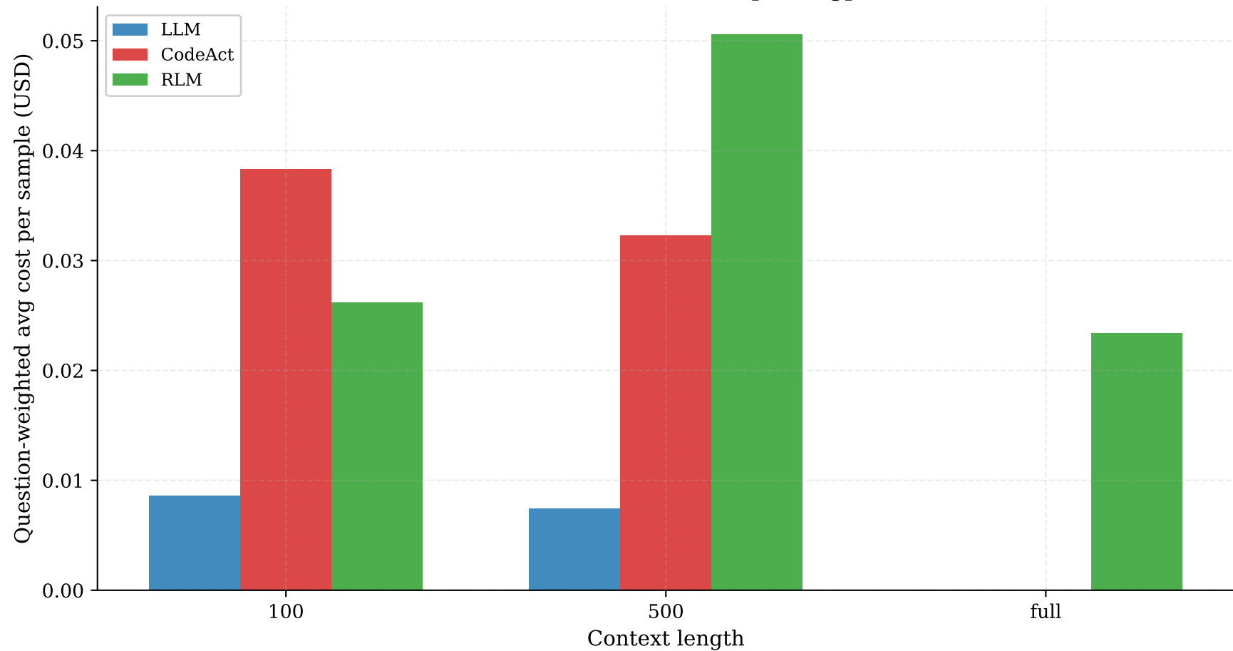
Tier4 overall cost vs context (openai/gpt-5-mini)
