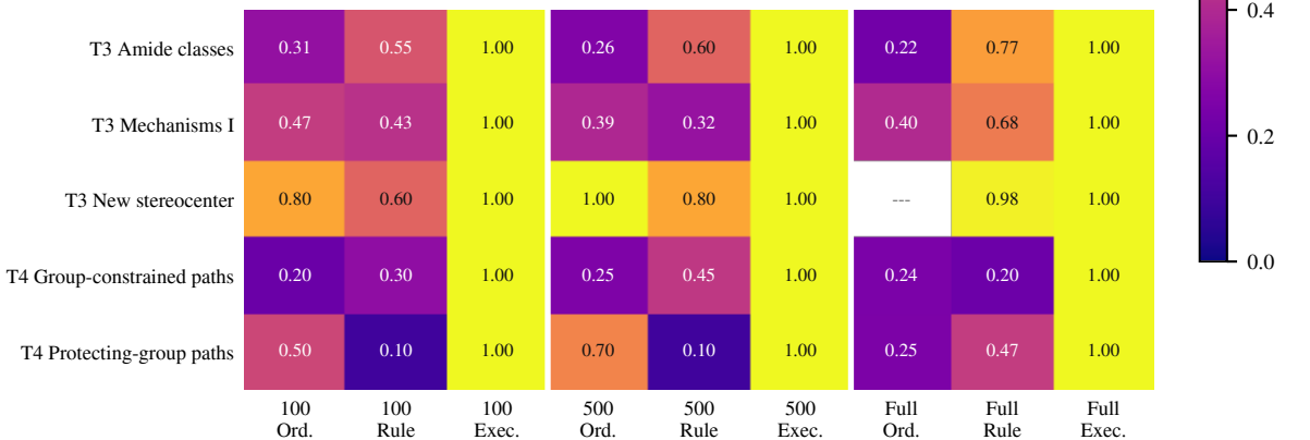
Claude Haiku 4.5
