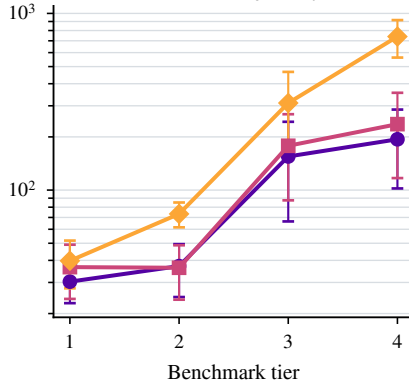
(e) Wall time (s) / trajectory
