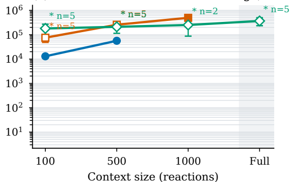
(c) Tier 3: Reaction-level reasoning ( n=35 )
