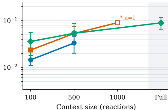
(c) Tier 3: Reaction-level reasoning ( n=35 )
