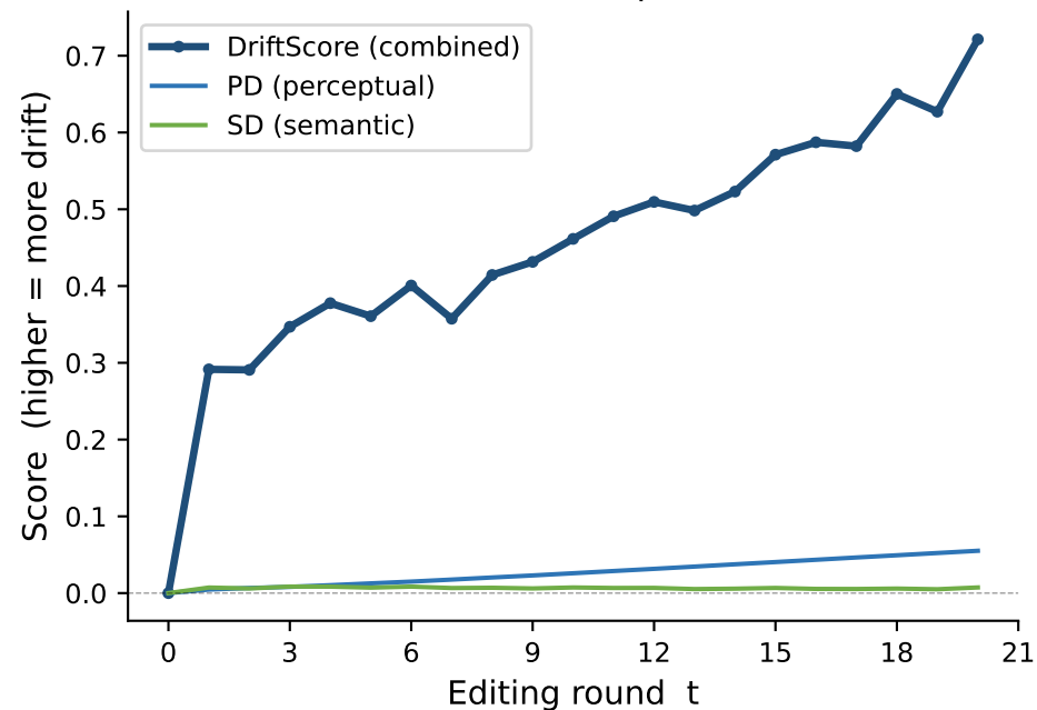
DriftScore Components
