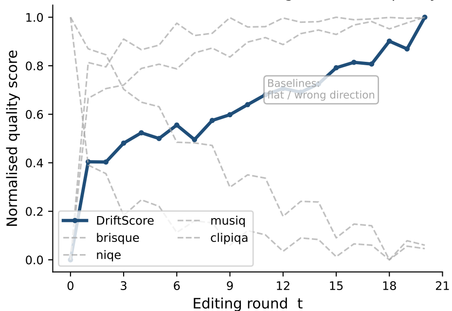
DriftScore vs. NR-IQA Baselines (scores normalised to [0,1], higher=better quality)
