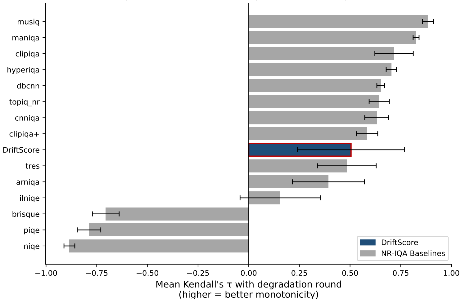
Degradation Detection: All Metrics (positive \tau = score correctly tracks increasing drift)
