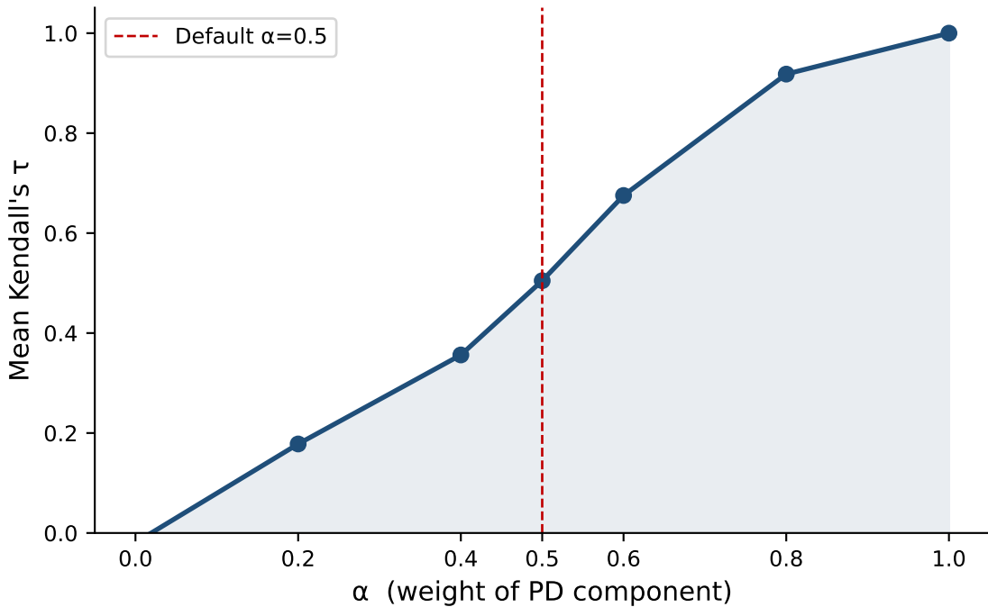
Alpha Ablation: Effect of PD vs. SD Balance
