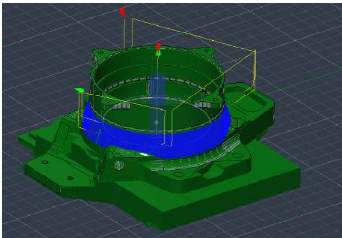
^ 5-Axis Finishing Flow Operation ^
