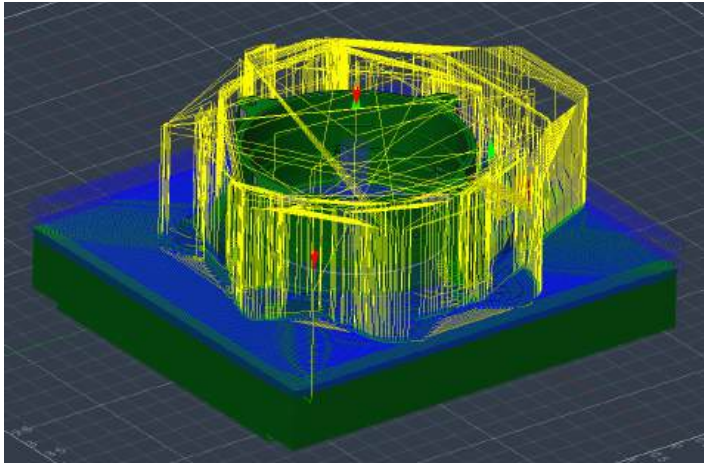
^ 5-Axis Roughing CAM Toolpaths for Rear Wheel Upright ^
