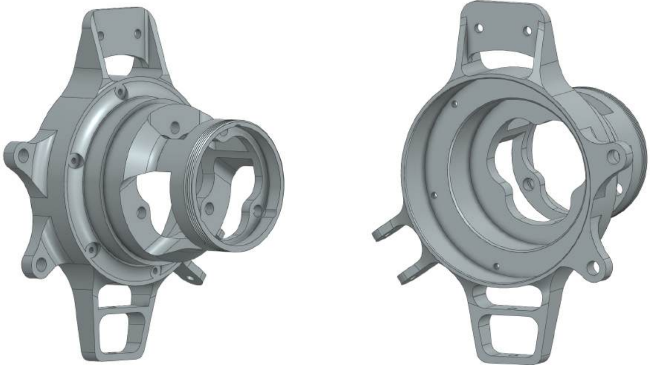
Unibody Upright & Planet Carrier Design
