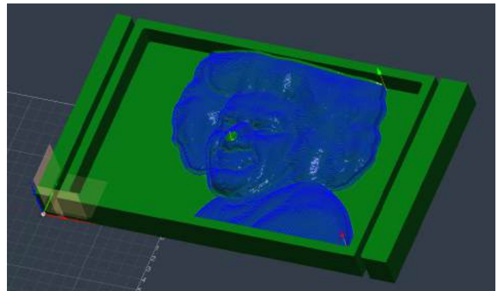
^ Created CNC Machining Toolpaths ^
