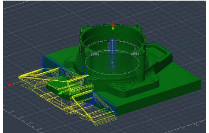
^ 5-Axis Roughing CAM Toolpaths for Rear Wheel Upright ^
