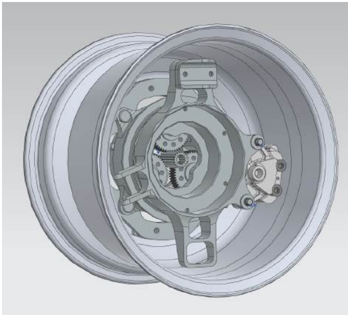
Full single wheel drivetrain assembly (without brake rotor, motor and accompanying peripheral parts)
