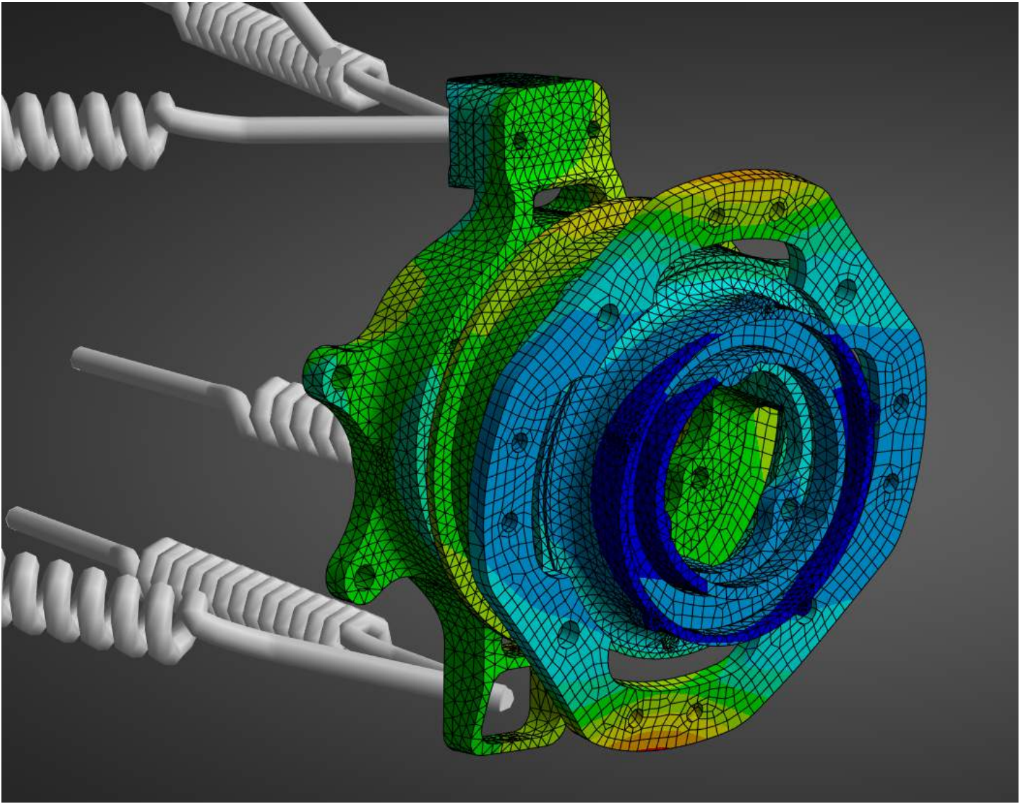
Rear Upright & Hub Group FEA
