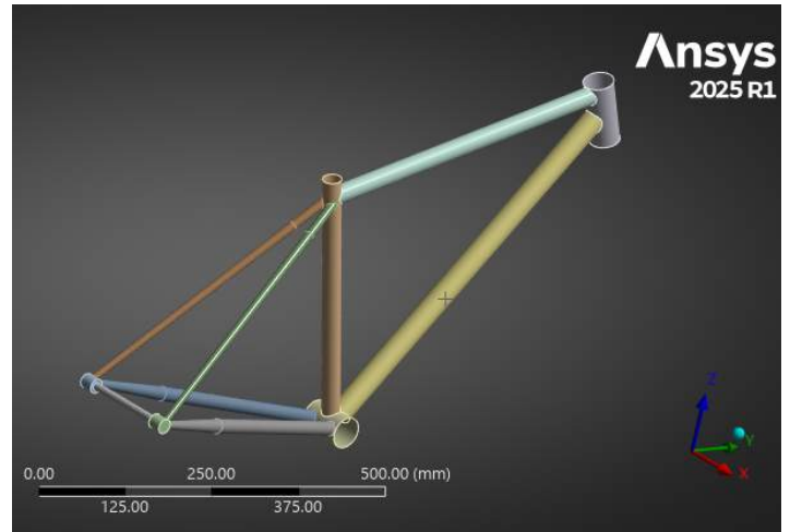
^ Frame Prepared for Meshing in Ansys ^
