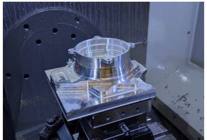
^ Upright After Completed 5-Axis Operation ^
