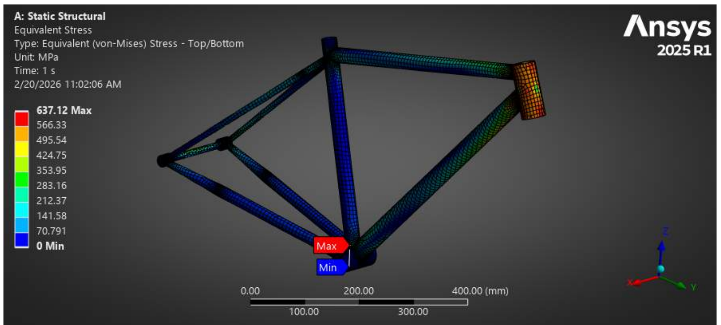
^ Von-Mises Equivalent Stress Results in Ansys ^
