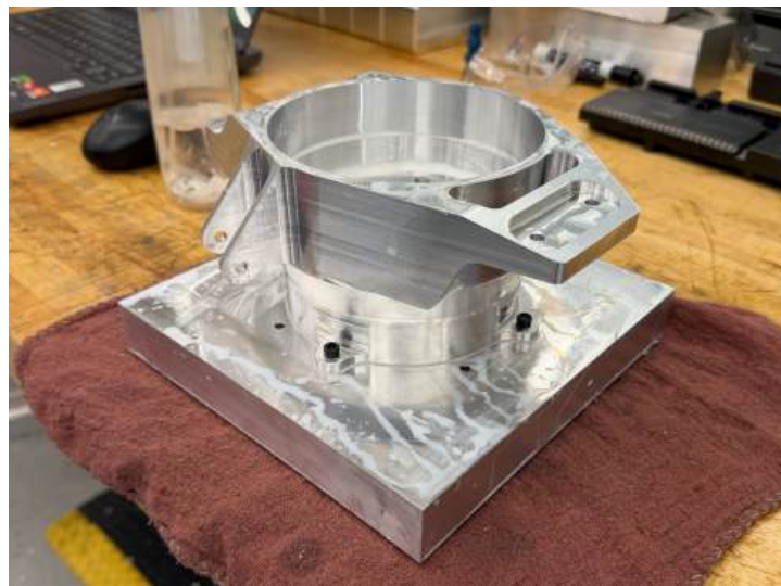
^ Upright After Final 3-Axis Operation ^
