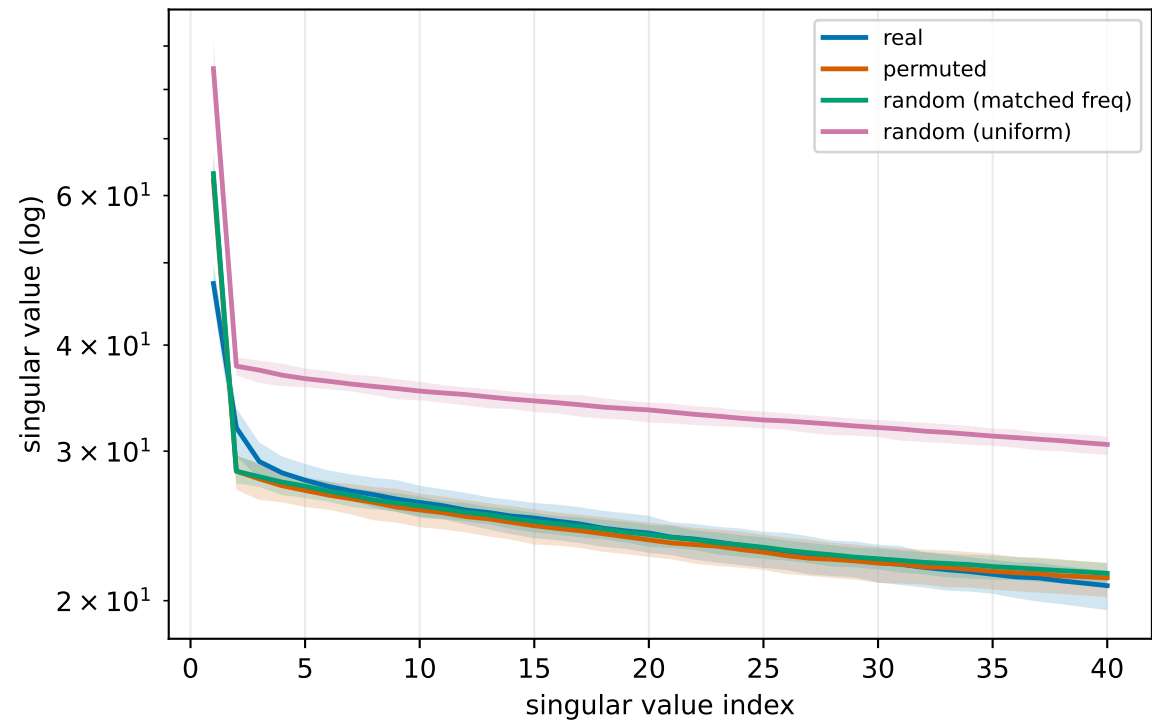
PPMI spectra with bootstrap 95% bands (B=50), real RR corpus vs controls
