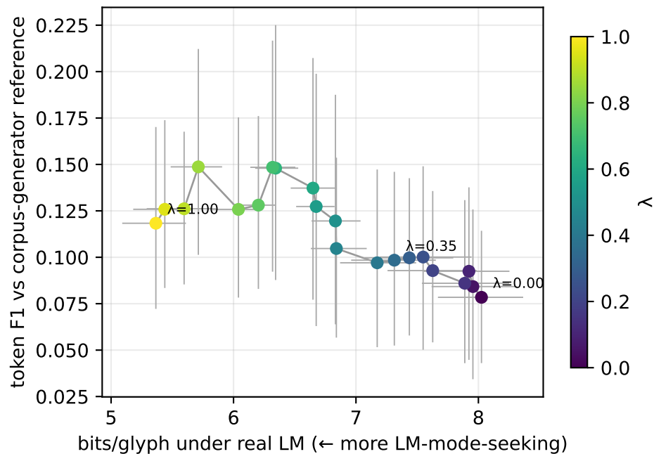
Fidelity–realism trade-off (95% bootstrap CIs)
