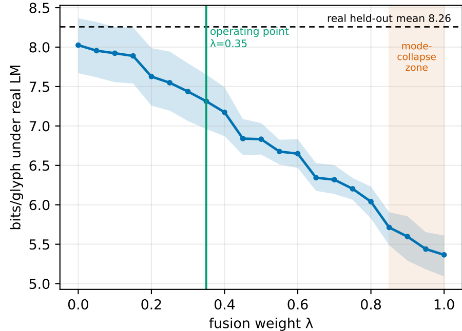
Monotone in \lambda , as predicted by Prop. P6(i)
