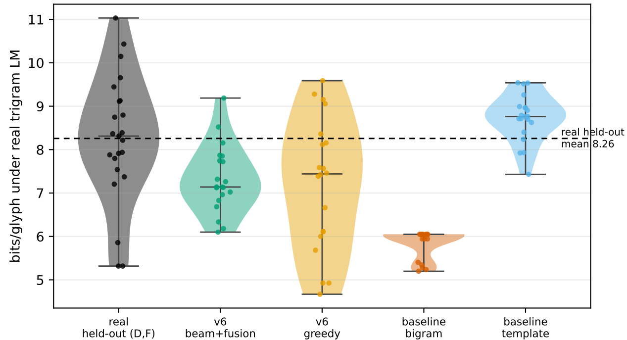
Per-line bits/glyph: real held-out vs generated outputs
