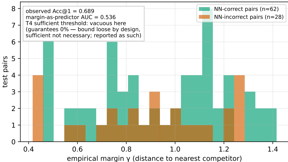
Margins vs. NN-matching correctness (synthetic anchor benchmark)
