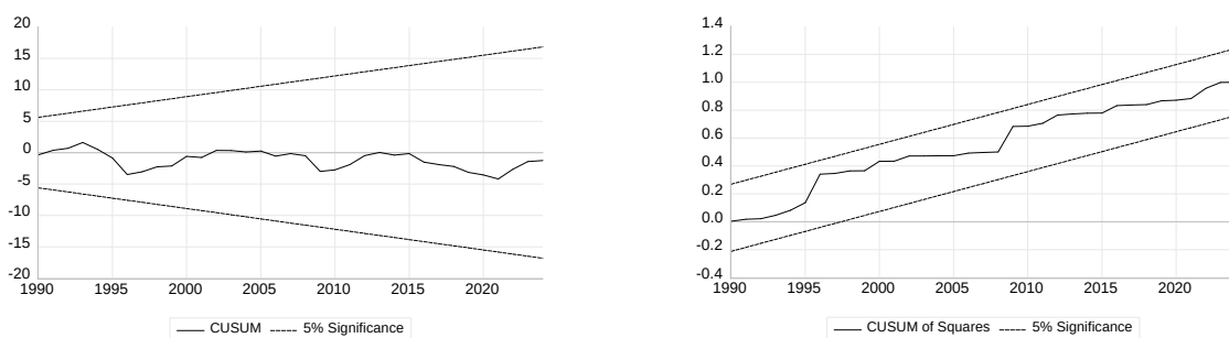
(a) CUSUM
