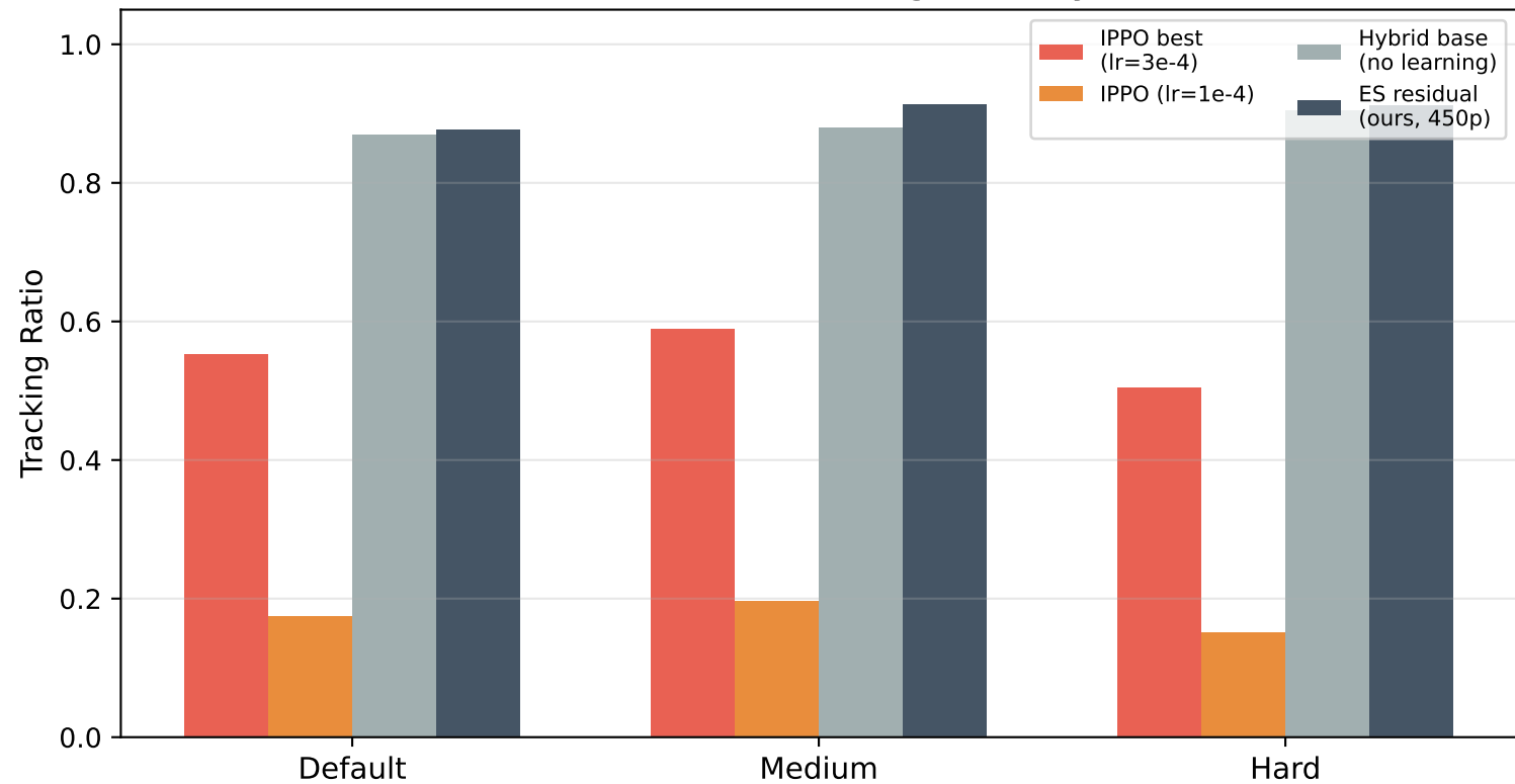
IPPO vs. ES Residual: Tracking Ratio by Scenario
