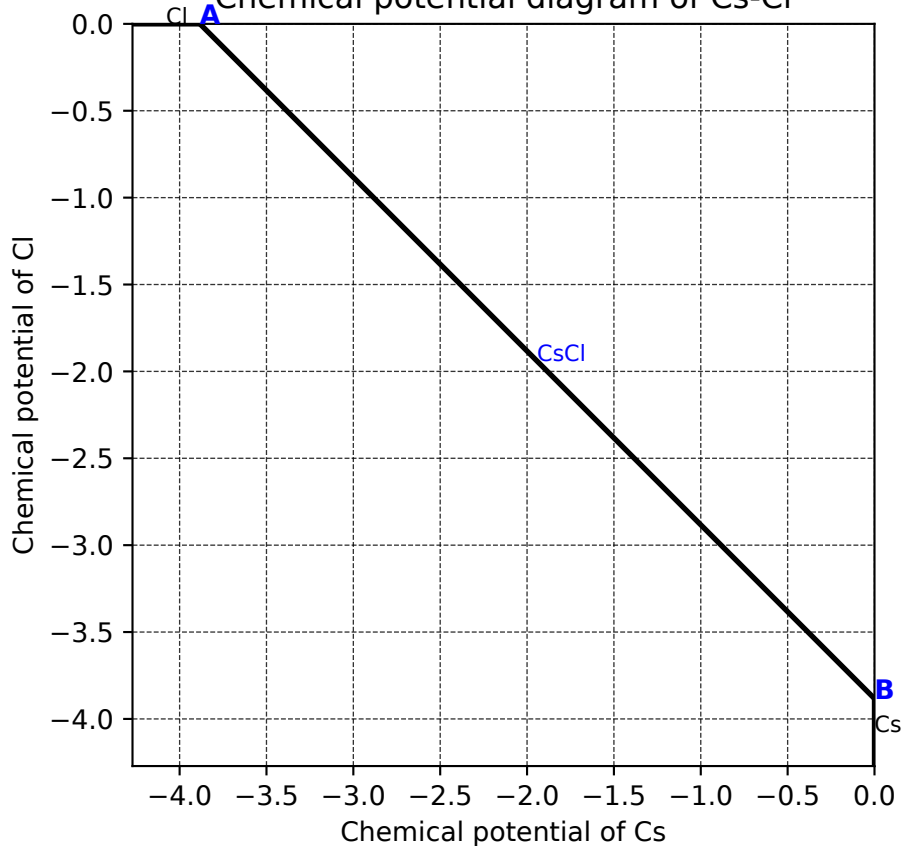
Chemical potential diagram of Cs-Cl
