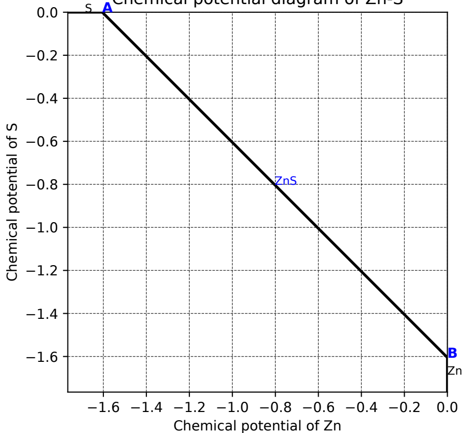
Chemical potential diagram of Zn-S
