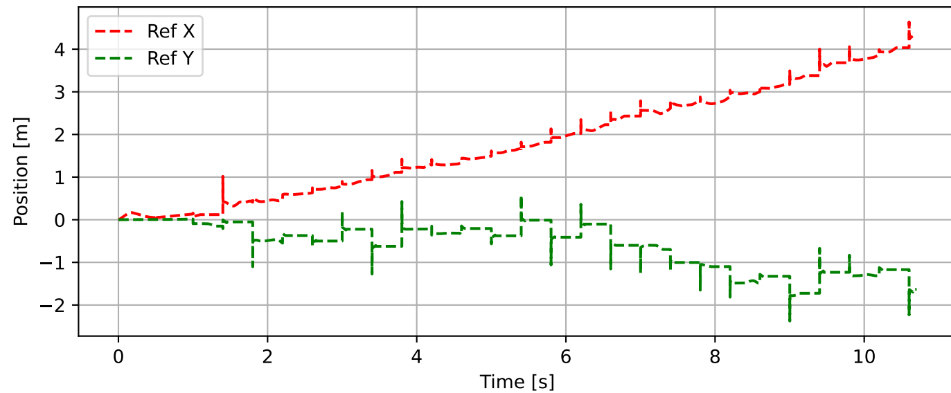
CoM Trajectory (Top View)
