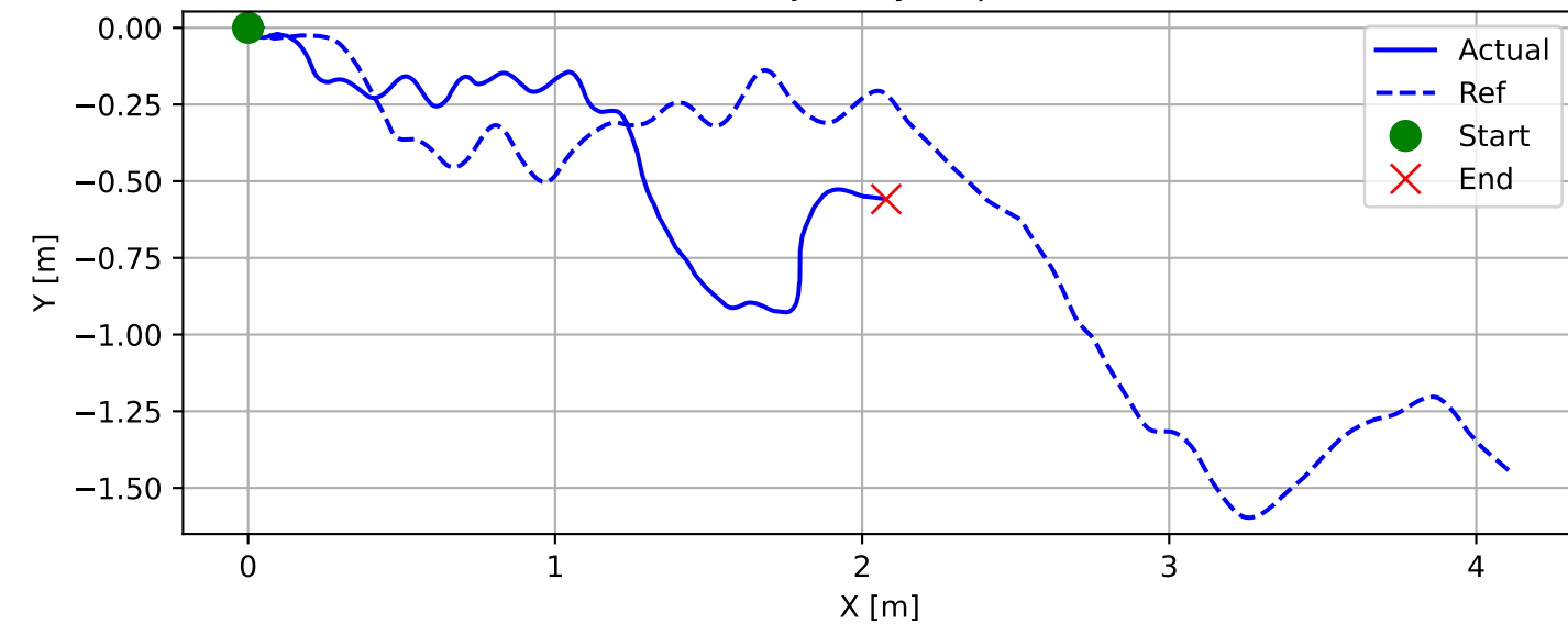
CoM Trajectory (Top View)
