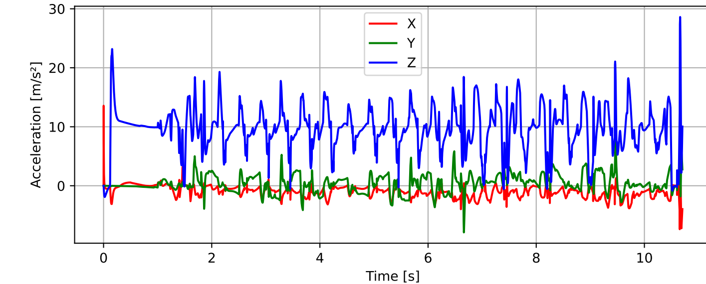
Base Acceleration
