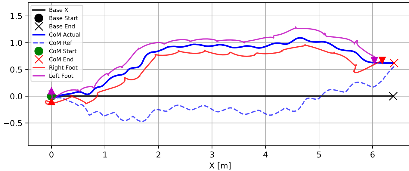
CoM &amp; Feet Trajectory (Top View)
